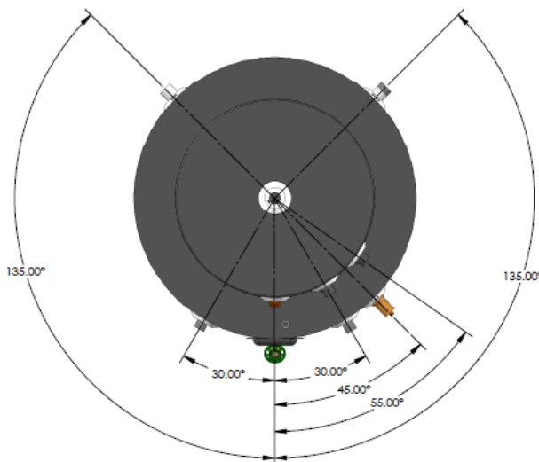
80 and 120 gallon overhead view of tank and Drainback reservoir
