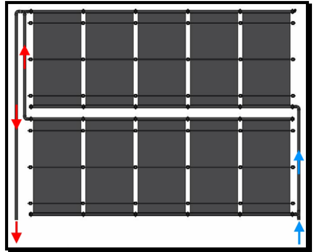
2. Double Row
