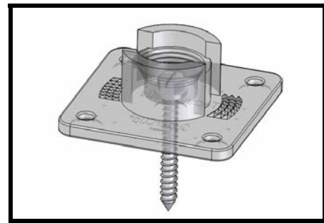
11. SuperClip Base
